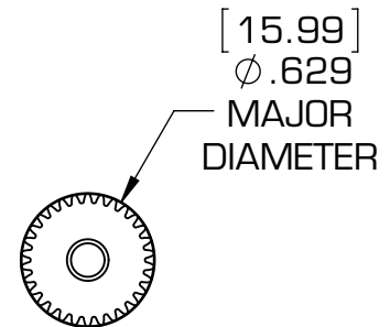
7:1 PLANET GEAR 30T
