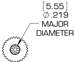
10:1 SUN GEAR 8T
