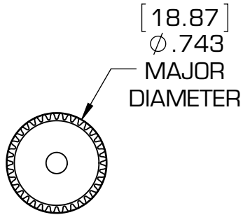
3:1 SUN GEAR 36T
